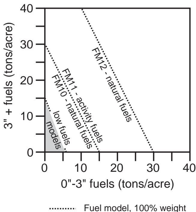
Figure 4.5 —If large and small fuels map to the shaded area, candidate fuel models are determined using the logic shown in figure 4.6. Otherwise, flame length is based on the distance to the closest fuel models, identified by the dashed lines, and on recent management (see “Model Description” chapter, section 2.4.8 for further details).
